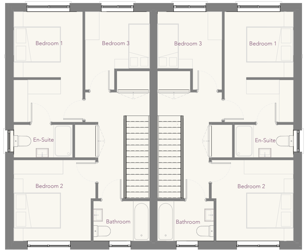
THE CITADEL First Floor Plan
