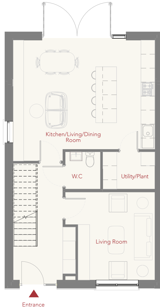
THE BASTION Ground Floor Plan
